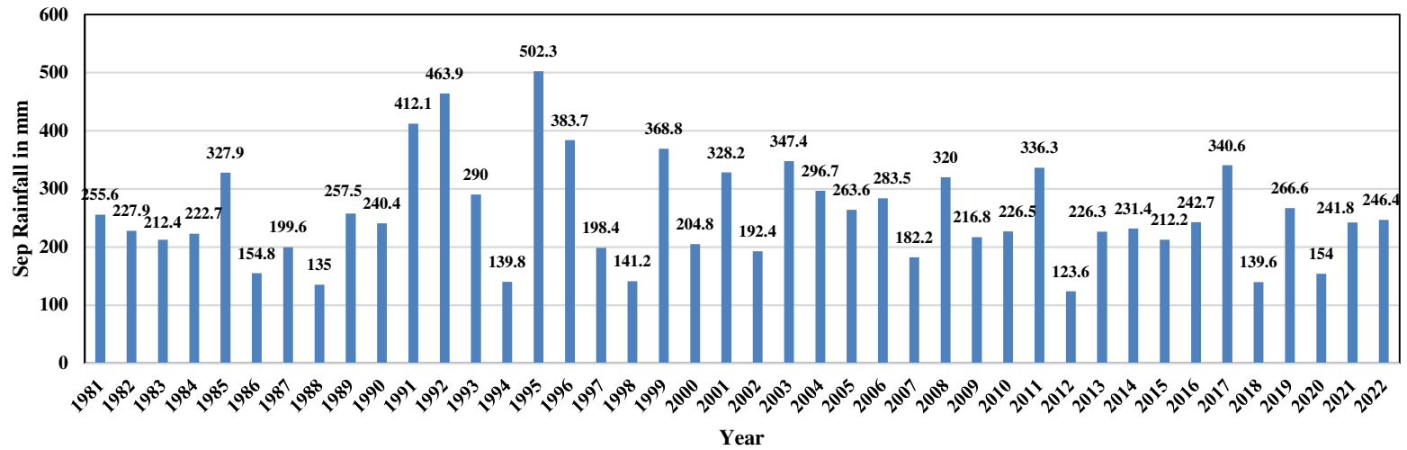
Rainfall of Kohima in September from 1981- 2022
