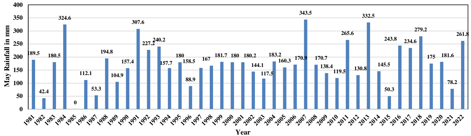
Rainfall of Kohima in May from 1981- 2022
