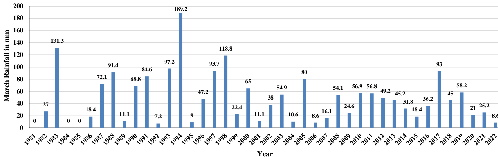
Rainfall of Kohima in March from 1981- 2022
