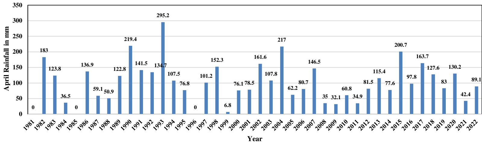
Rainfall of Kohima in April from 1981- 2022
