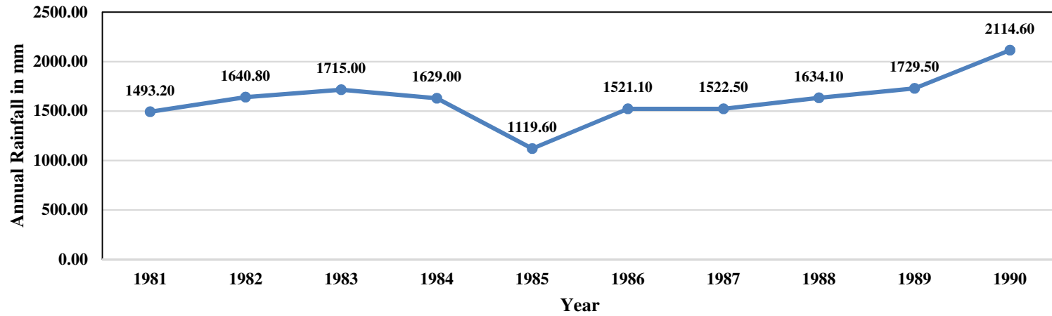
Fig 3 (a): Decadal Variation of Kohima Rainfall (1981 to 1990)
