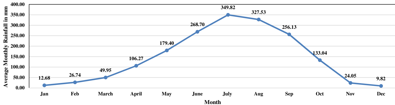
Figure 1 (b): Average Monthly Variation of Rainfall in mm for Kohima (1981- 2022)
