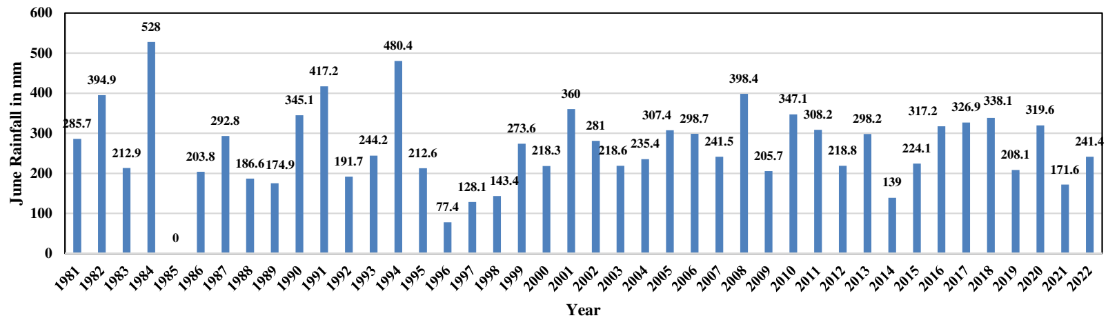
Rainfall of Kohima in June from 1981- 2022
