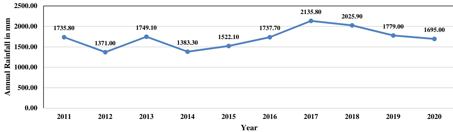
Fig 3 (d): Decadal Variation of Kohima Rainfall (2011 to 2020)
