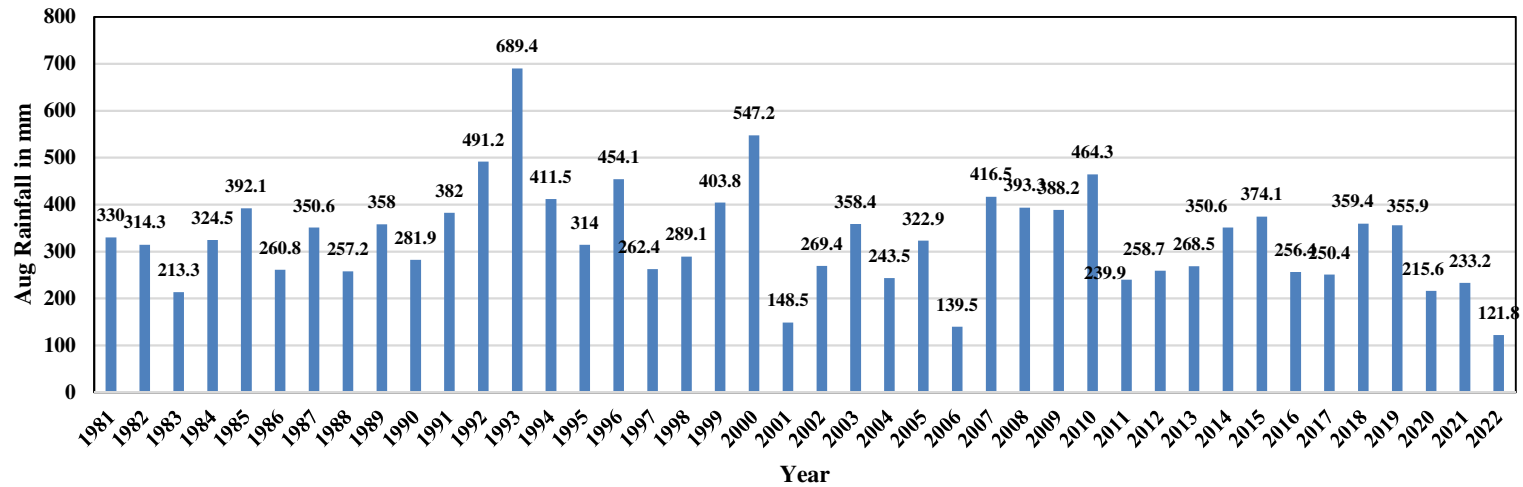
Rainfall of Kohima in August from 1981- 2022
