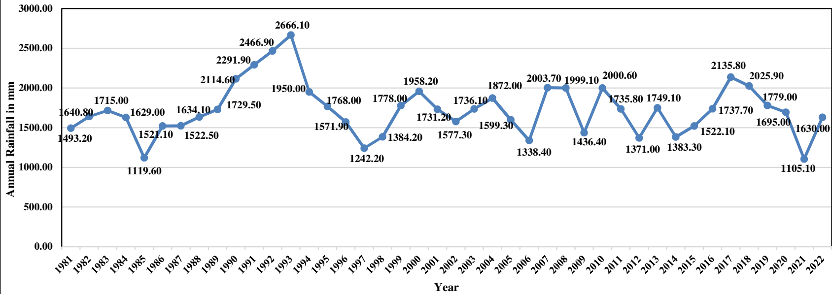
Figure 1 (a): Variation of Kohima Annual Rainfall in mm for 42 Years from 1981- 2022
