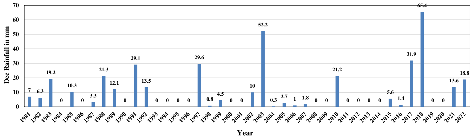
Rainfall of Kohima in December from 1981- 2022
