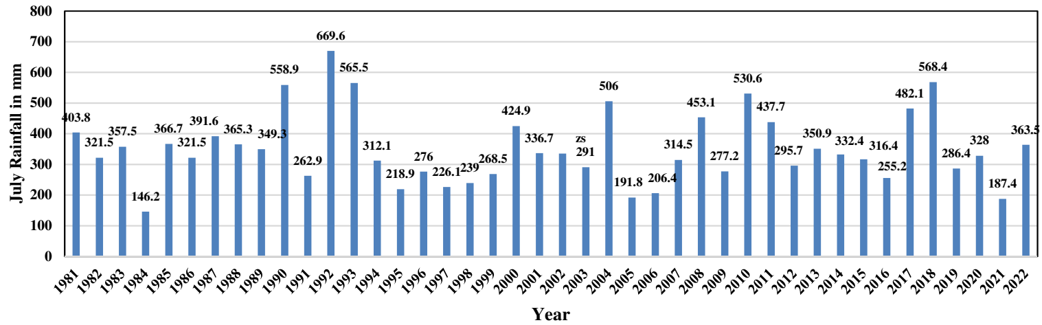
Rainfall of Kohima in July from 1981- 2022
