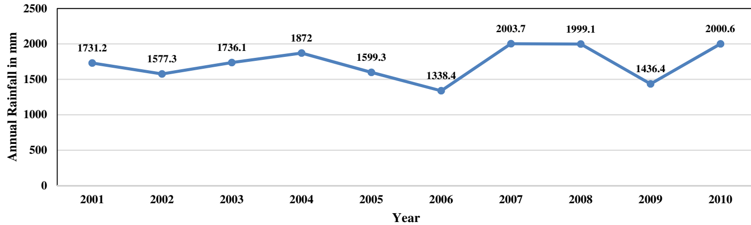
Fig 3 (c): Decadal Variation of Kohima Rainfall (2001 to 2010)
