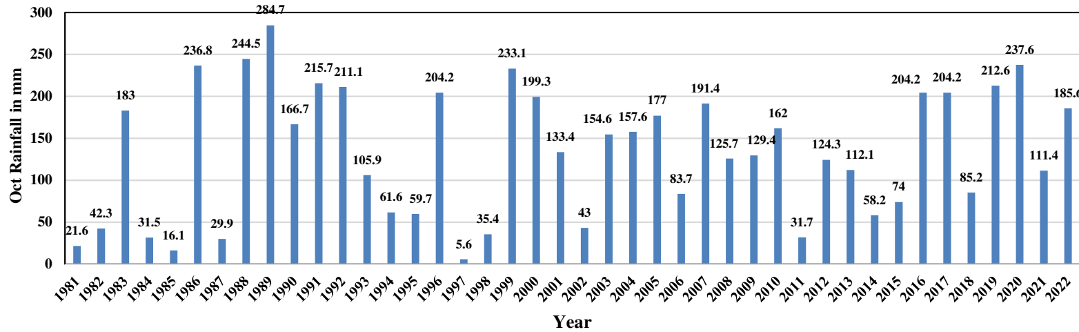
Rainfall of Kohima in October from 1981- 2022
