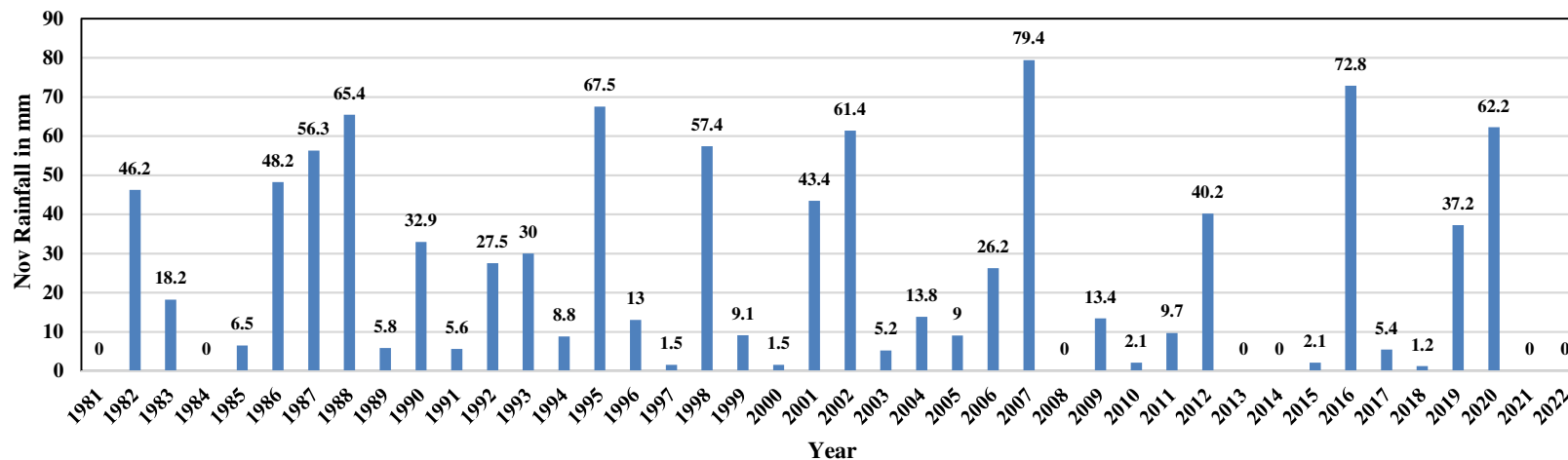
Rainfall of Kohima in November from 1981- 2022
