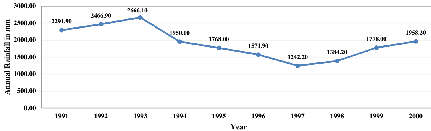
Fig 3 (b): Decadal Variation of Kohima Rainfall (1991 to 2000)
